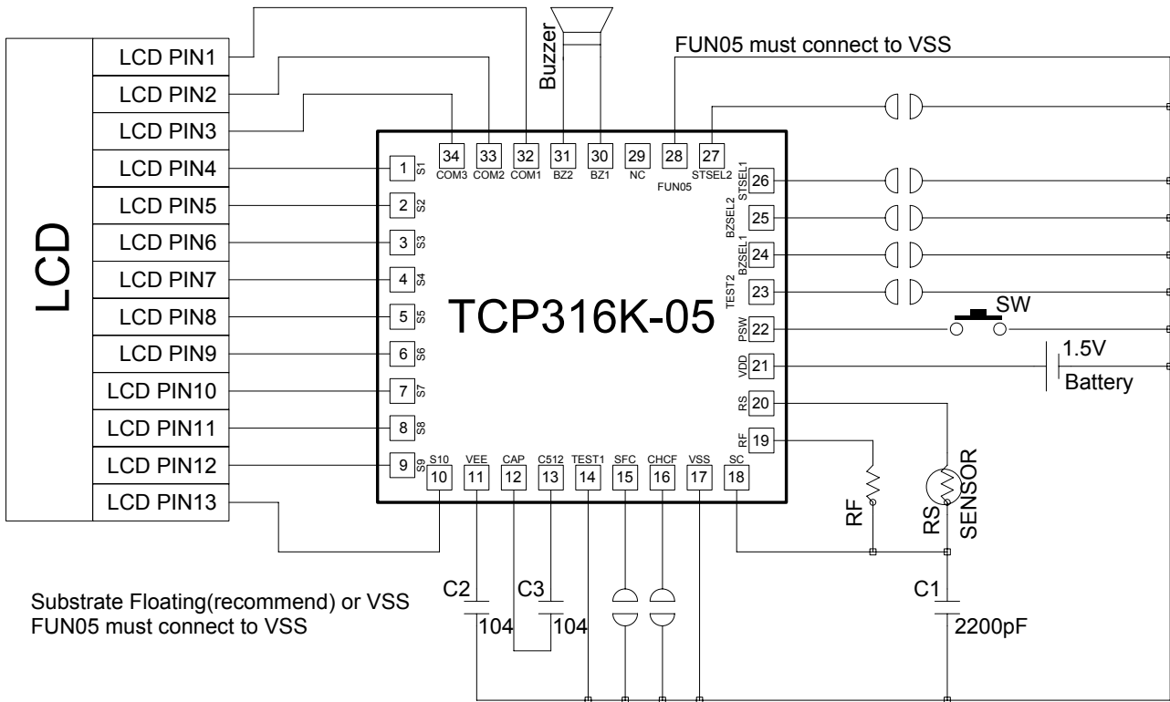
TCP316K-05A/TCP316K-05B Application Circuit
